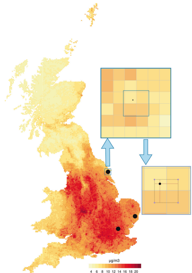
Fig. 1 The maps display PM_{2.5} levels on a specific day over Great Britain, with three locations (large black dots) that represent the residential addresses of a specific subject (ID 2 in Table 1). The magnified area on top represents the exact location at higher resolution, surrounded by the four nearest centroids (small indigo dots) of the overlaid PM_{2.5} grid. Without interpolation, the residential exposure value (small black dot) would be represented by the value of the nearest centroid. The magnified area below illustrates the process of reconstructing the residential value as a bilinear interpolation of the four nearest centroids.
