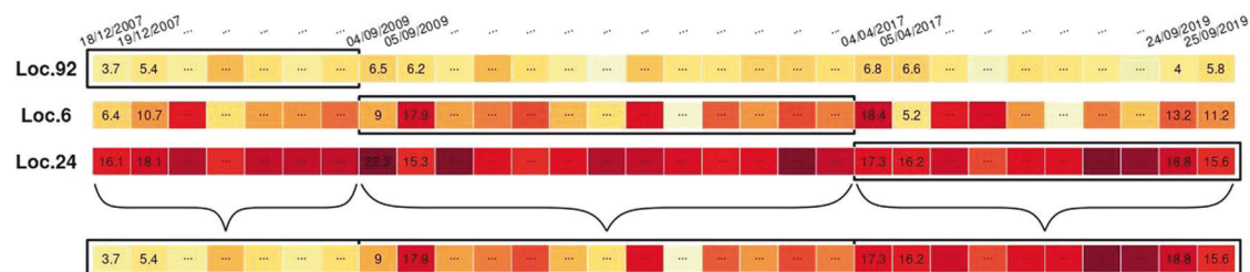
Fig. 2 The top three series represent the sequences of daily exposures at the residential addresses of subject ID 2. At the bottom, the final subject-specific exposure series is assembled by concatenating the three series above based on the respective residential periods.
